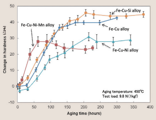
Fig. 3: Effect of solute elements on the hardening of thermally aged RPV model alloys
