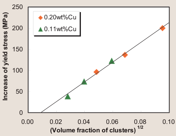
Fig. 2: Relationship between the microstructure (volume fraction) and the mechanical property (yield stress)
