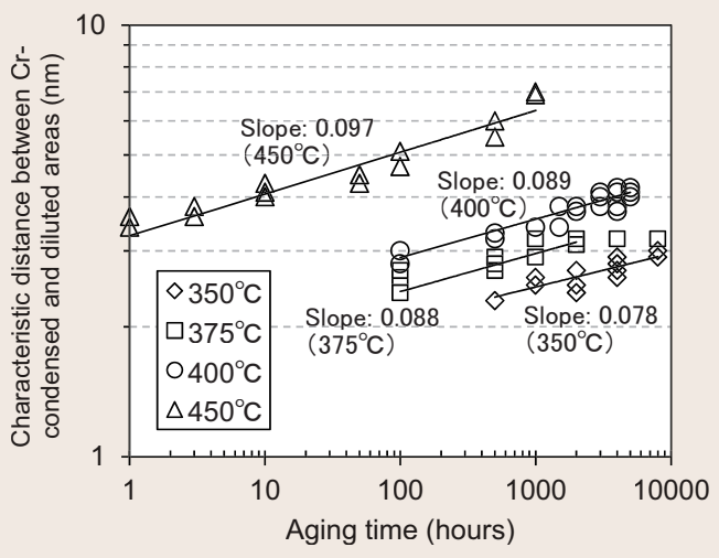
(b) Representative length of Cr-rich phase decomposition
