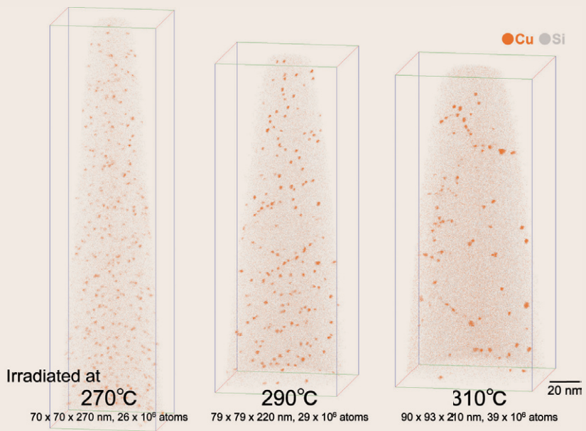
Fig. 1: Effect of irradiation temperature on the solute atom cluster formation in Cu-containing (0.2 wt% Cu) material
