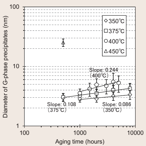
(a) Size of G-phase precipitates
