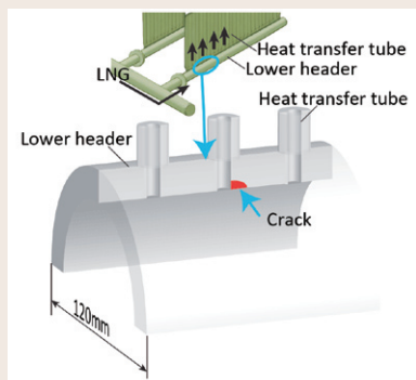
(a) Structure of an open rack vaporizer
