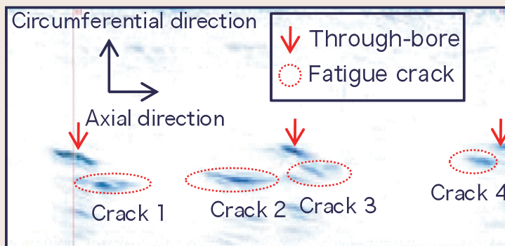
(b) Example of the detection of cracks in an open rack vaporizer
