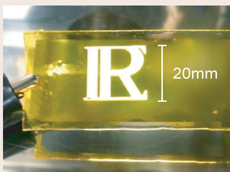
Fig. 2: Prototype device of the new light-emitting device made of ionic liquid and light-emitting organic polymer
