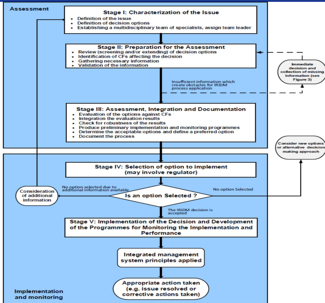
FIG. 3. IRIDM workflow.
